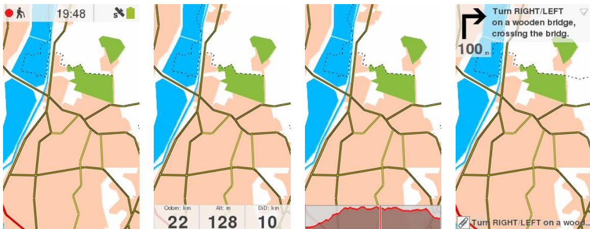
STATUS BAR
